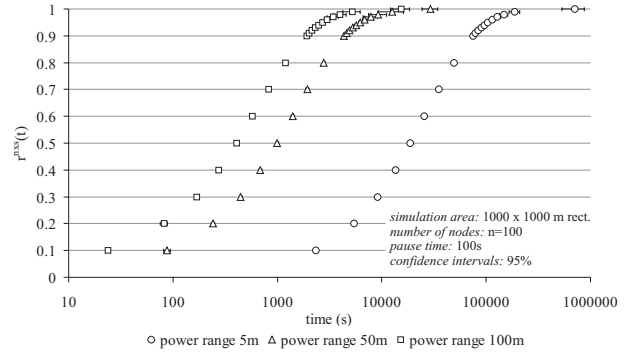
Figure 8: Convergence r^{n \times s}(t) with the random waypoint model on a 1000 \times 1000 m rectangle for n = 100 , s = 99 , and for several node power ranges.
