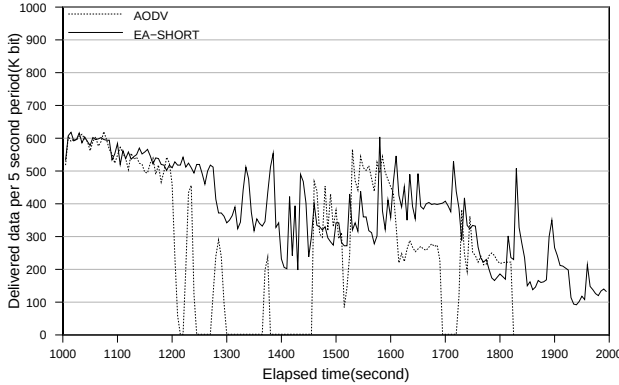
Figure 13: Time-line of network capacity(Delivered data per 5 second period).
