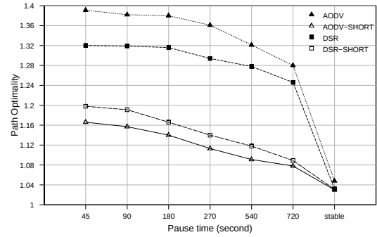
Figure 9: Path Optimality.
