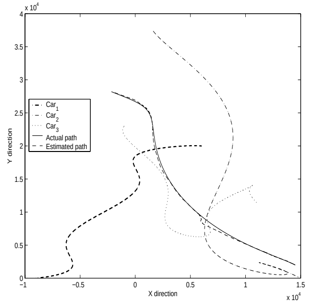
Figure 4: Trajectories of the cars and the mobile user for the case of dual base station measuring
