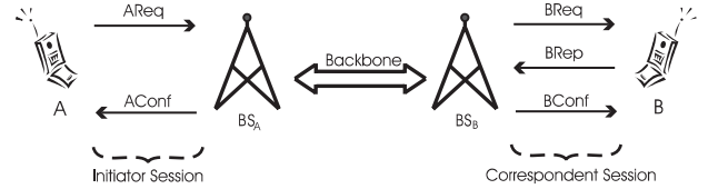
Figure 1: The session setup phase
