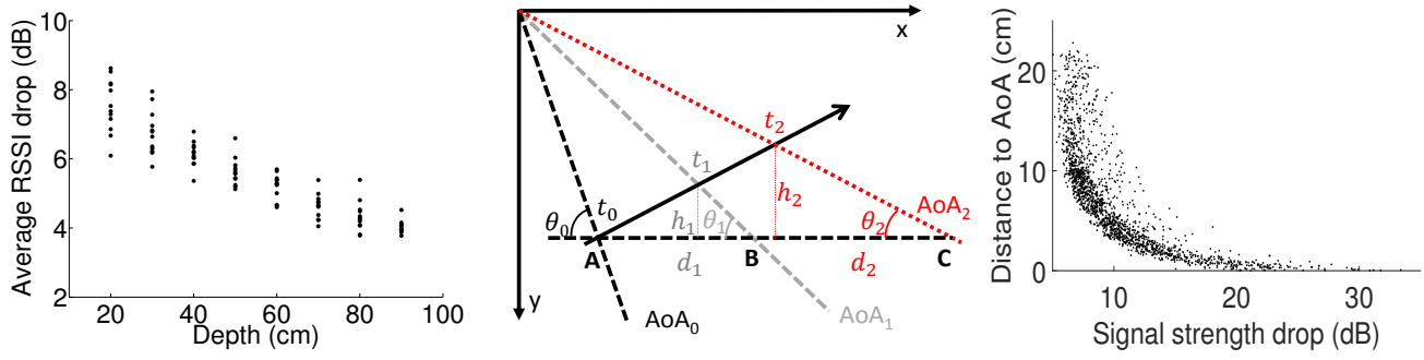
Figure 7: (a) Average RSSI drop across all AoAs vs. depth of the hand from the WiDraw receiver. 25 locations in the same 2x2 square feet area were picked uniformly at each depth value. (b) Estimating depth changes by utilizing the time duration between AoA minima. The user's hand crossed 3 AoAs ( AoA_0 , AoA_1 , and AoA_2 ) in a 3D movement. The trajectories of the hand movement and 3 AoAs were projected to the 2D X-Y plane. (c) The drop in signal strength of an AoA is proportional to the hand's distance from the AoA.
