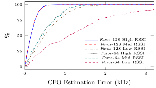
Figure 8: Cumulative distribution functions of CFO estimation error with various sequence lengths and RSSIs. Faros provides frequency synchronization within 800 Hz at up to -75 dBm.
