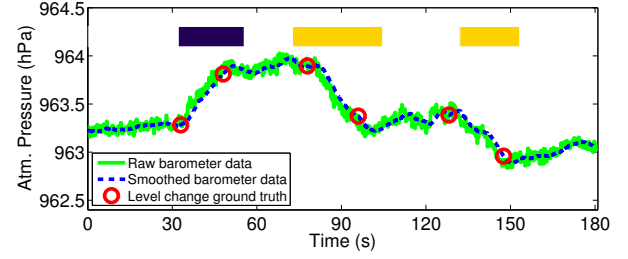
Figure 10: Data processing for level change detection.
