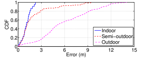
Figure 18: Tracking error of the walking progress estimator.
