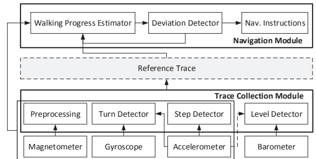
Figure 1: Architecture of FOLLOWME.
