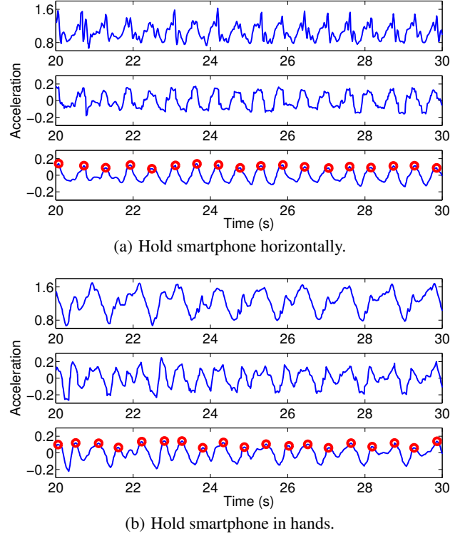
Figure 9: Data processing for step detection.
