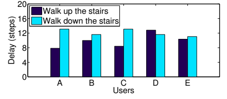
Figure 15: Delay of level-change detection.
