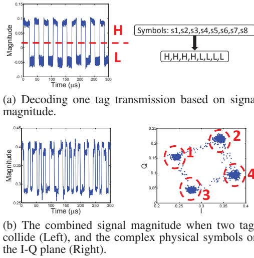
Figure 1: Decoding tag signals from single and multiple concurrent transmissions.
