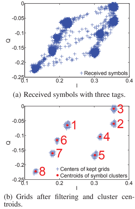
Figure 2: Symbol clustering.
