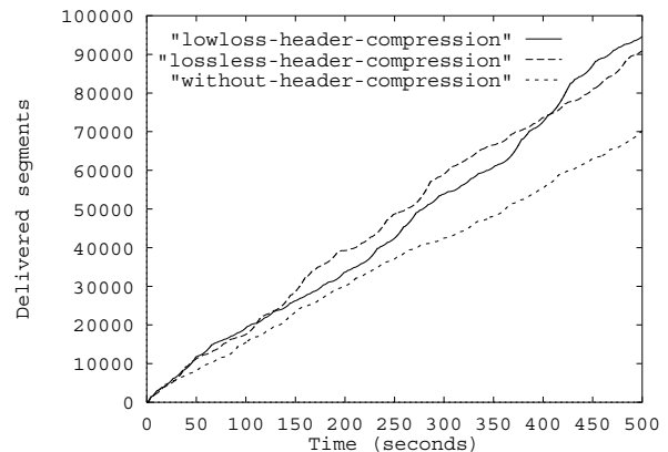
Figure 18: Delivered 512 byte segments over WLAN topology with bit-error rate 2 \times 10^{-7} .
