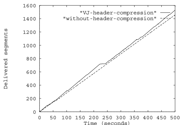
Figure 11: Number of 512 byte segments delivered across Modem topology with bit-error rate 2 \times 10^{-6} .
