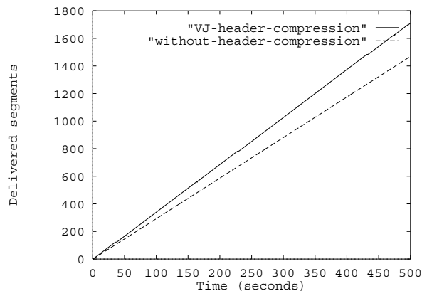
Figure 10: Number of 512 byte segments delivered across Modem topology with bit-error rate 2 \times 10^{-7} .
