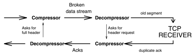
Figure 17: Header request mechanism.
